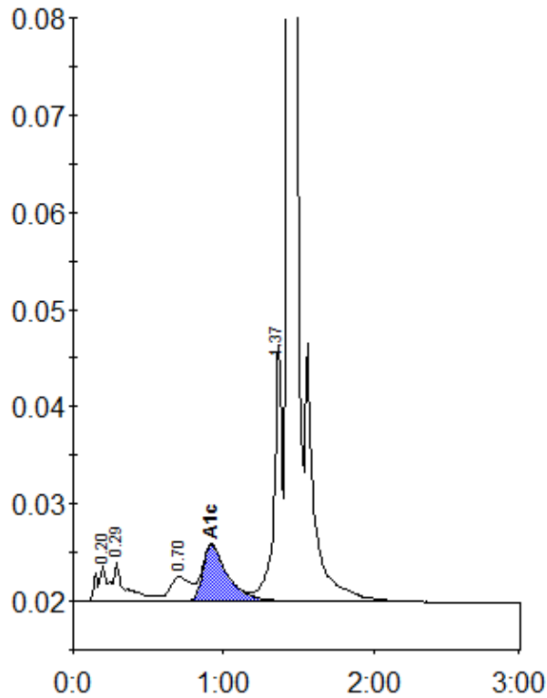
Peak table - ID: 10681652
